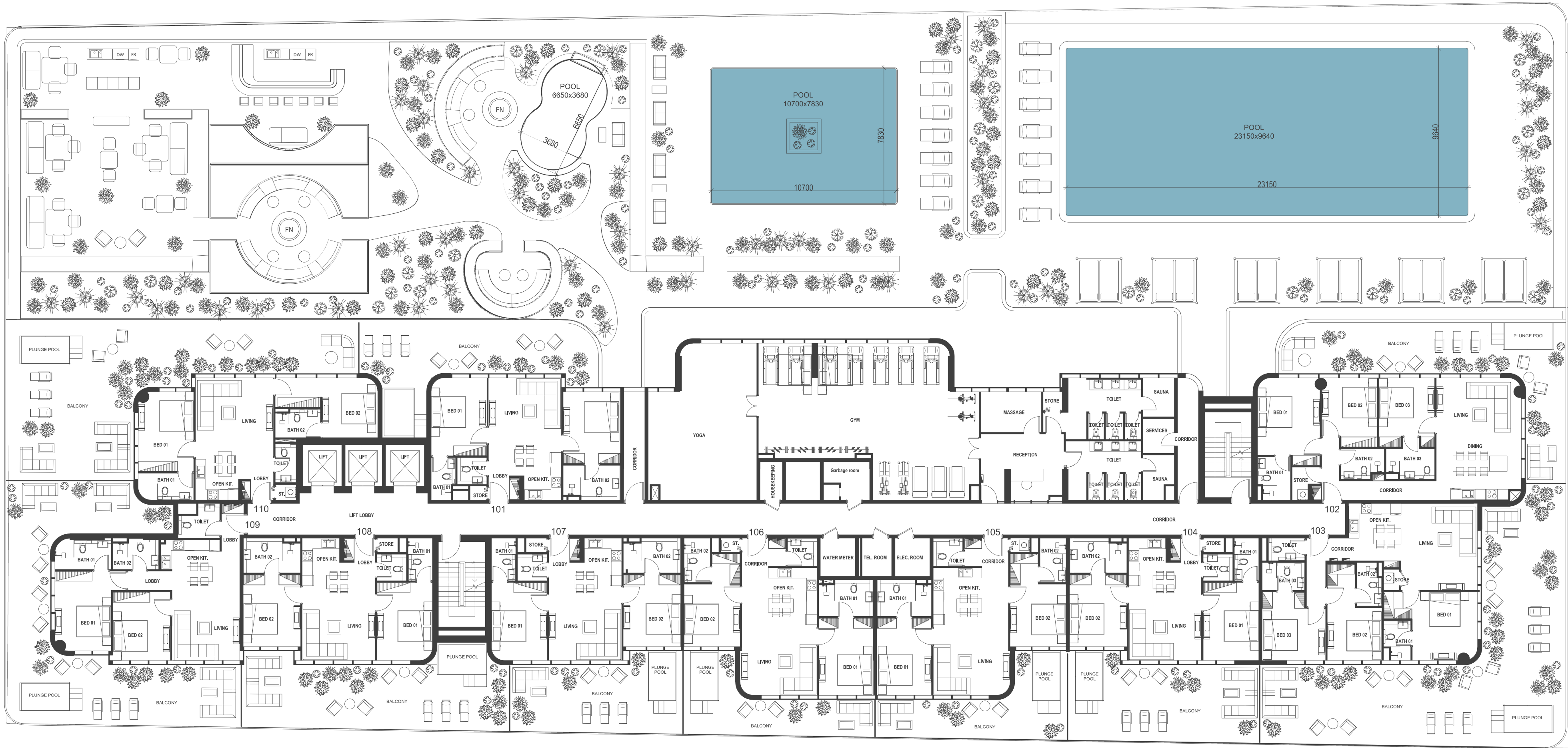
1-ST FLOOR
