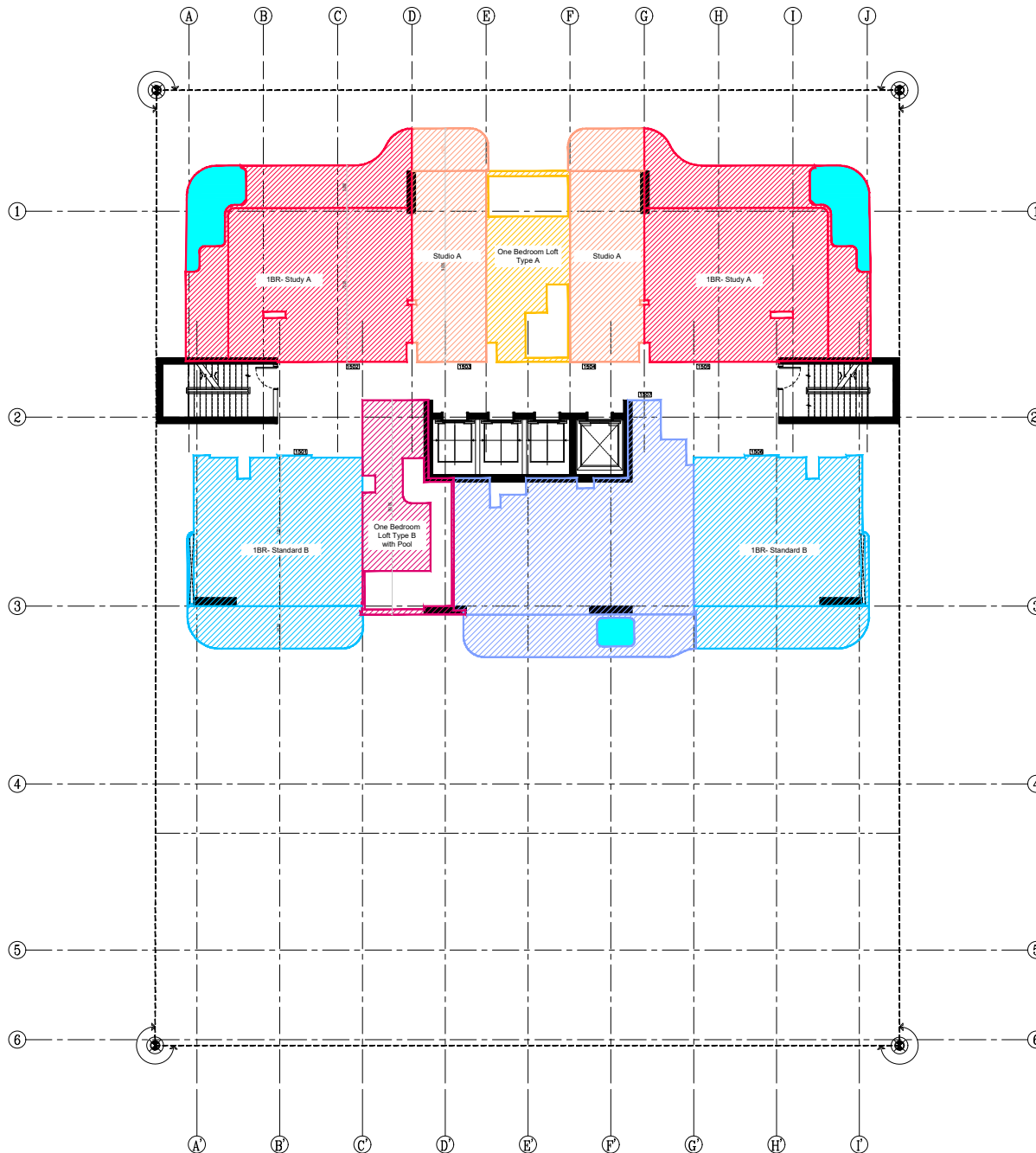
15TH FLOOR PLAN
