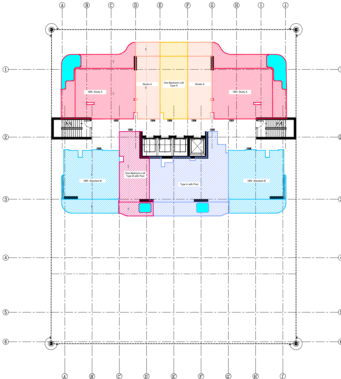
16TH FLOOR PLAN
