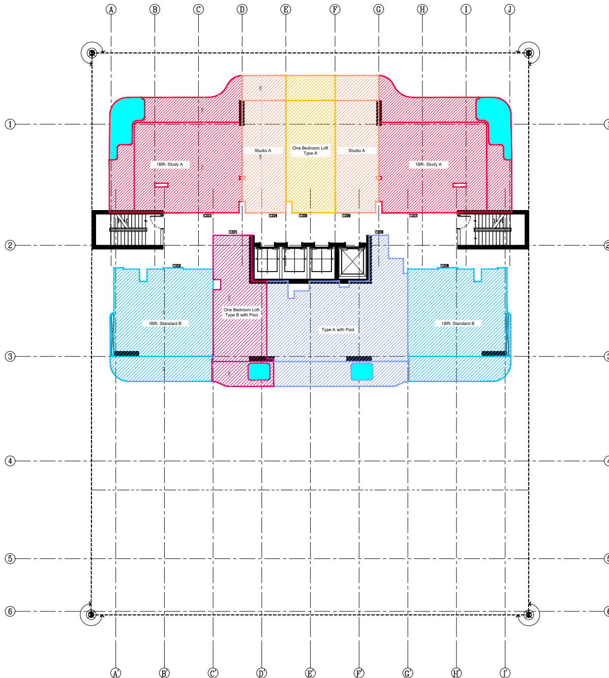
12TH FLOOR PLAN
