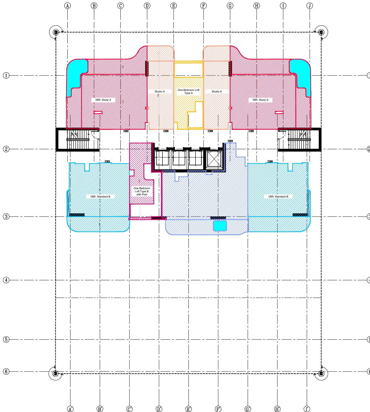
13TH FLOOR PLAN
