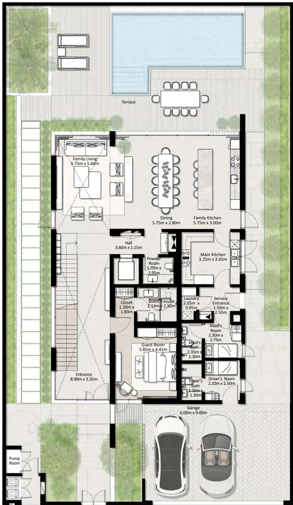
GROUND FLOOR
